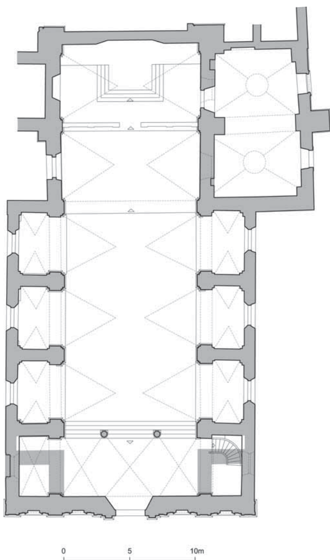
Crkva sv. Katarine, tlocrt na donjoj razini s naznakom neizvedenih zvonika (arhitektonska snimka: I. Tenšek, I. Valjato-Vrus) St Catherine's church, ground plan of the lower level, with an outline of the unrealised belfries
